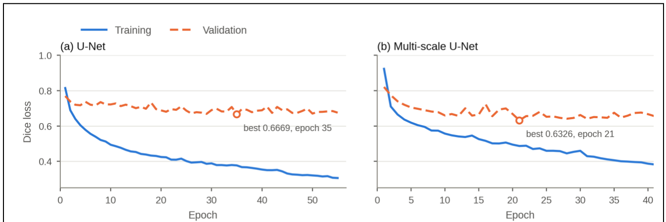
Fig. 6. Training and validation Dice-loss curves of (a) the conventional U-Net and (b) the proposed Multi-scale U-Net with data augmentation. The vertical axis limits, the line styles and the marker convention are those of Fig. 5, so the two training conditions can be compared directly.
