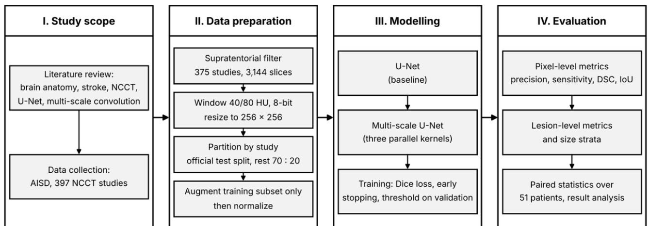
Fig. 1. Overall workflow of the proposed acute ischemic stroke infarct segmentation framework, including NCCT data acquisition, preprocessing, patient-level partitioning, model training, and performance evaluation. The four labelled stages of the diagram are study scope, data preparation, modelling and evaluation.
