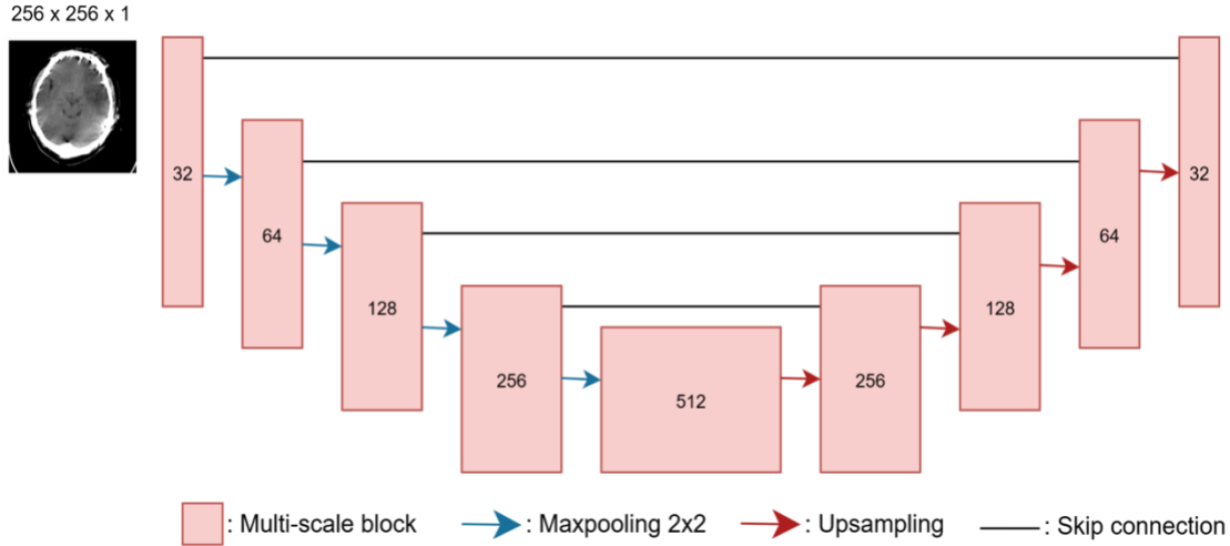
Fig. 4. Detailed architecture of the proposed Multi-scale U-Net for acute ischemic stroke infarct segmentation, showing encoder-decoder stages, skip connections, multi-scale convolution blocks, and output segmentation masks. The input is one 256 \times 256 \times 1 NCCT slice. The five encoder stages carry 32, 64, 128, 256 and 512 channels, each a multi-scale block of Fig. 3 followed by 2 \times 2 max pooling, and the decoder mirrors them with transposed convolutions and skip connections. A final 1 \times 1 convolution with a sigmoid returns a 256 \times 256 \times 1 probability map, which the threshold of Eq. (19) turns into the output segmentation mask.
