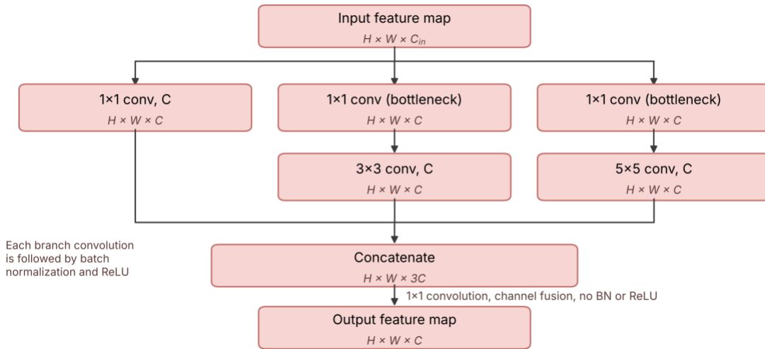
Fig. 3. Architecture of the proposed multi-scale convolution block incorporating parallel 1 \times 1 , 3 \times 3 , and 5 \times 5 convolutional kernels, feature concatenation, and channel fusion. The input feature map carries C_{in} channels at H \times W .
