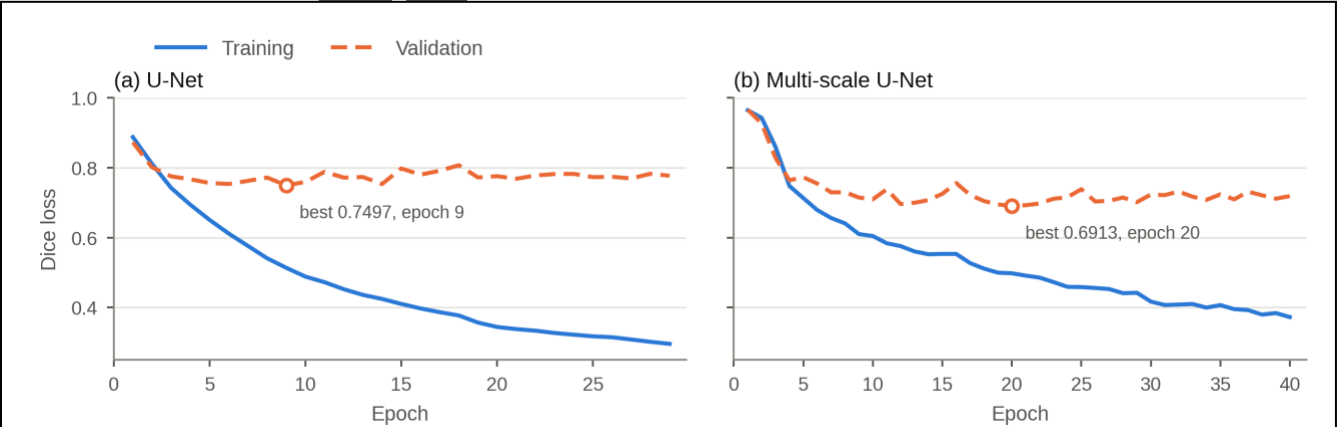
Fig. 5. Training and validation Dice-loss curves of (a) the conventional U-Net and (b) the proposed Multi-scale U-Net without data augmentation. The solid line is the training loss and the dashed line the validation loss. The open circle on each validation curve marks the epoch of lowest validation loss, whose weights were kept for testing. Both panels use the same vertical scale and the same line styles; the horizontal axis spans the epochs each run completed before early stopping.
